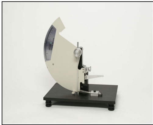
The Model ME-800 Elmendorf Tear Tester with Manual Sample Clamps and Integral Sample Cutting Knife Mechanism
